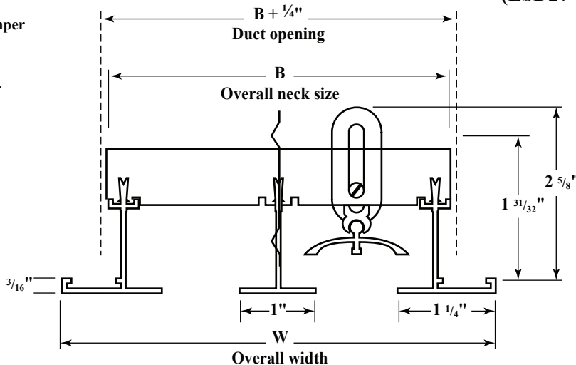
LSD20 / LSD27 (LSD27 two slots shown here)
