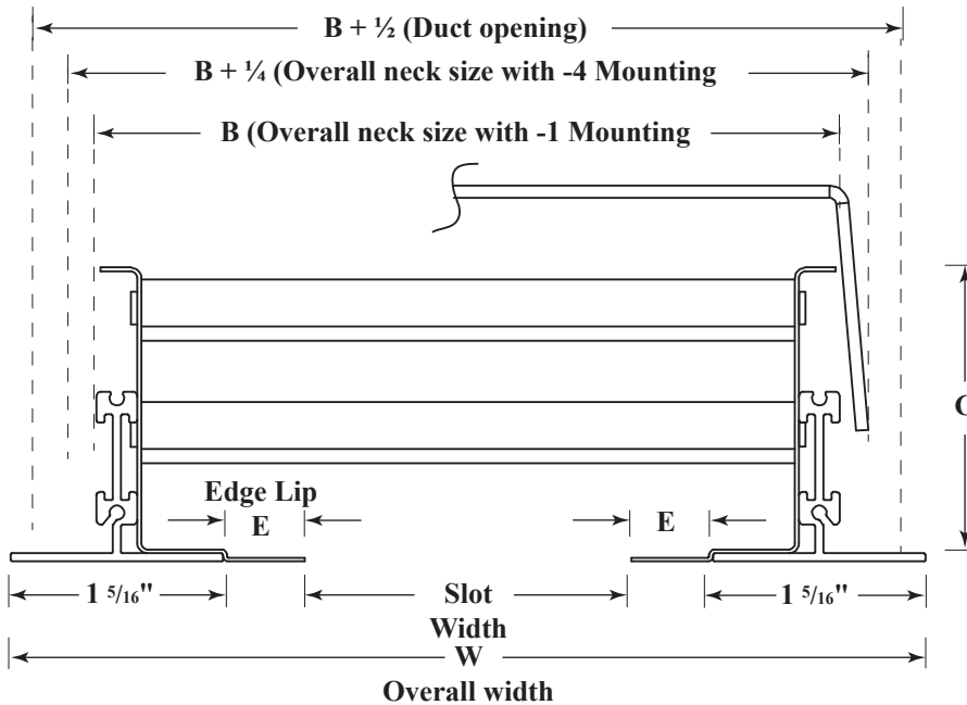
LFB10 without pattern-control damper
